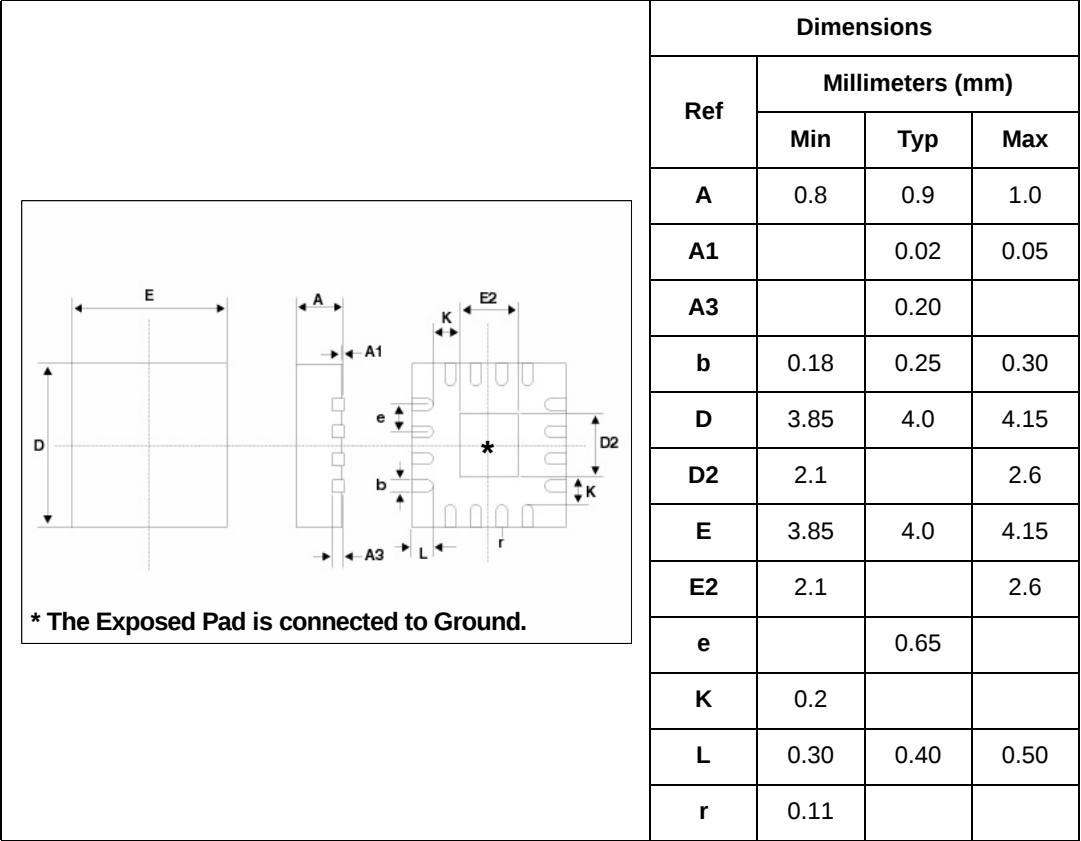
Figure 71. QFN16 4x4mm package mechanical data
