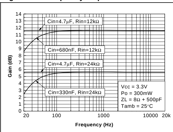
Figure 55. Frequency response
