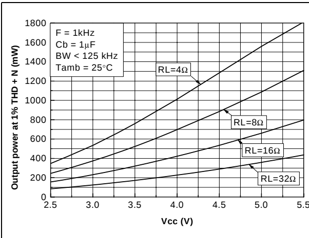
Figure 58. Output power vs. power supply voltage
