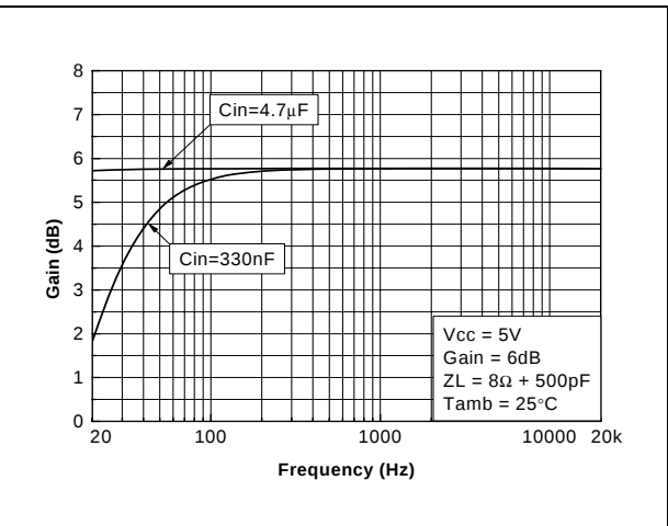
Figure 53. Frequency response
