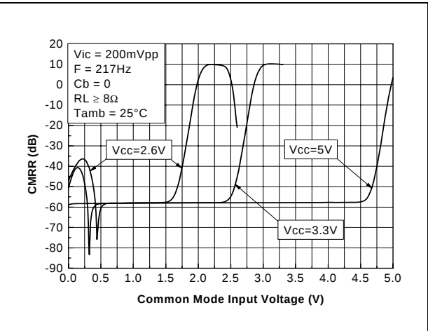
Figure 45. CMRR vs. common mode input voltage
