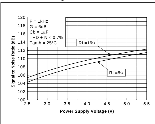
Figure 54. SNR vs. power supply voltage with unweighted filter
