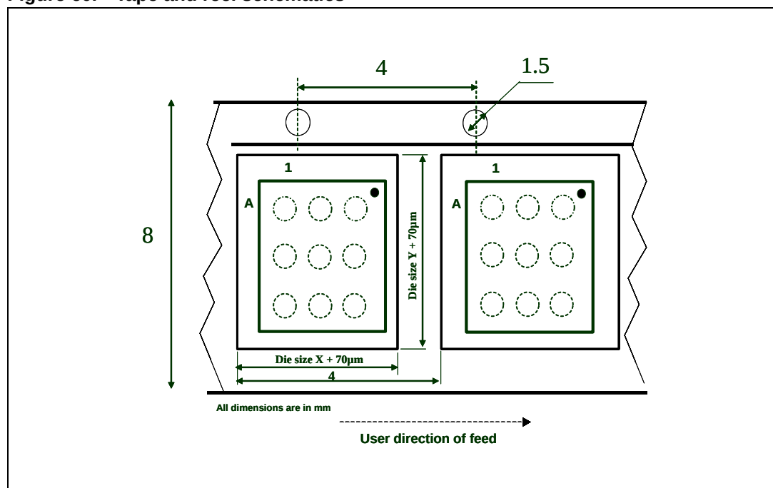
Figure 60. Tape and reel schematics
