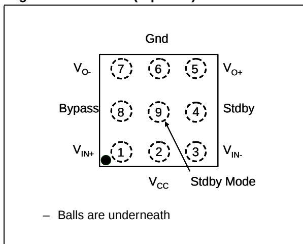
Figure 61. Pin out (top view)
