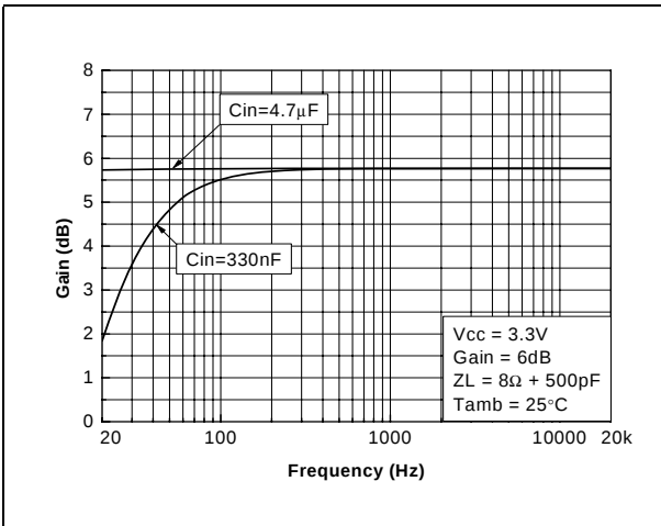
Figure 52. Frequency response
