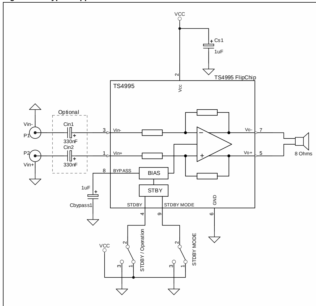
Figure 1. Typical application
