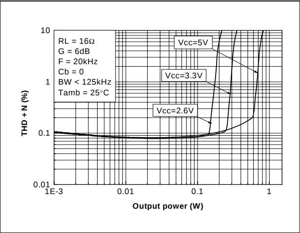
Figure 17. THD+N vs. output power
