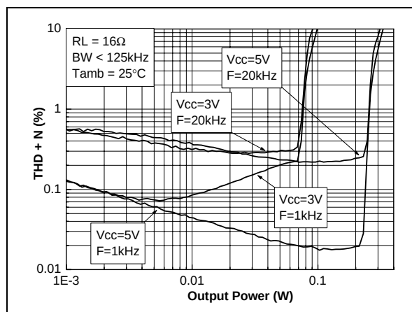
Figure 8: HDout THD+N vs. output power (Output modes 4, 5 G=+12dB)
