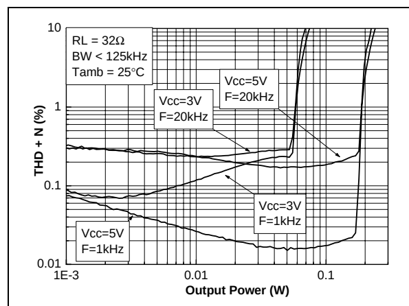
Figure 11: HDout THD+N vs. output power (Output modes 4, 5 G=+6dB)
