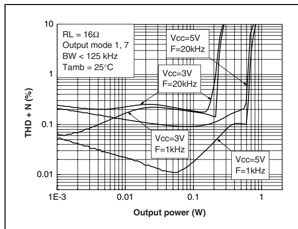
Figure 5: Spkout THD+N vs. output power (output modes 1, 7)
