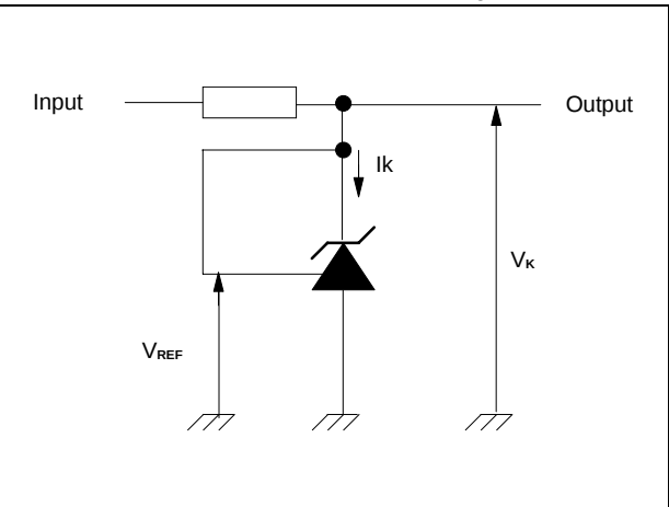
Figure 2. Test circuit for V_K = V_{ref}
