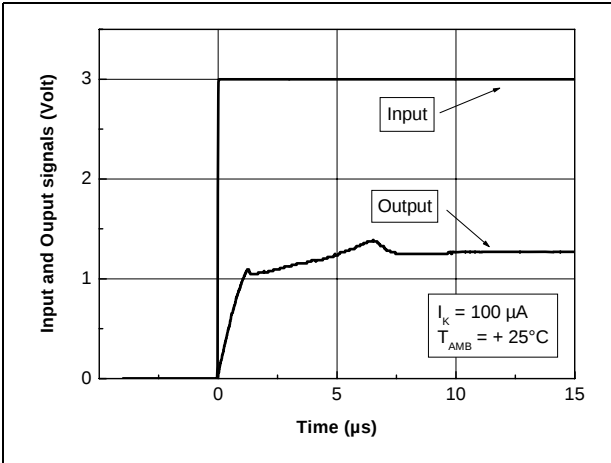
Figure 15. Pulse response at I_K = 100\mu A
