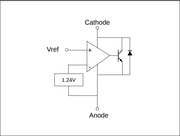
Figure 20. Block diagram
