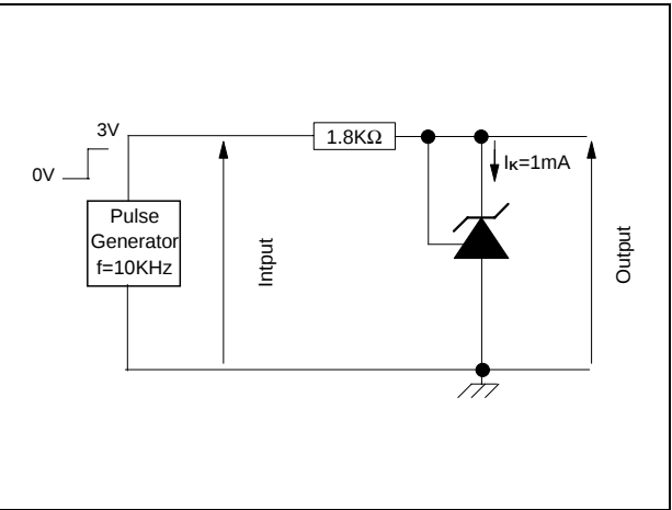
Figure 14. Test circuit for pulse response at I_K = 1\text{ mA}
