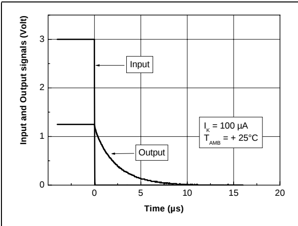
Figure 17. Pulse response at I_K = 100\mu A
