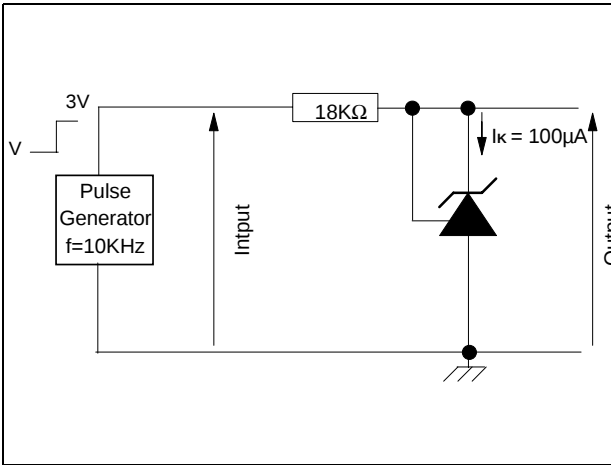
Figure 13. Test circuit for pulse response at I_K=100\mu A
