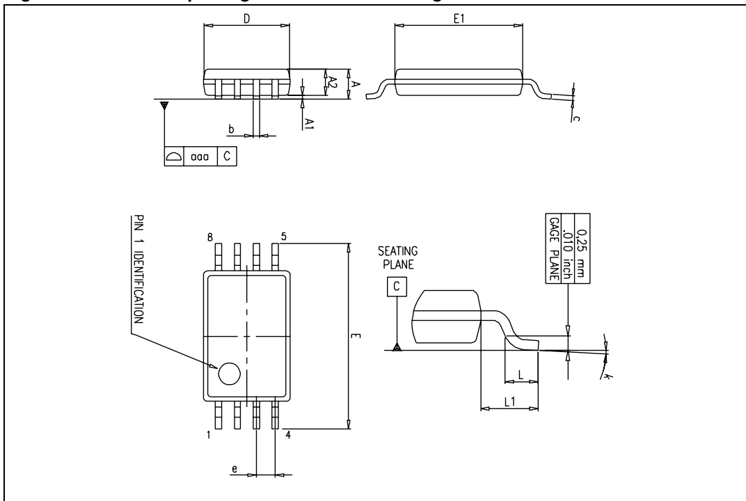
Figure 4. TSSOP8 package mechanical drawing
