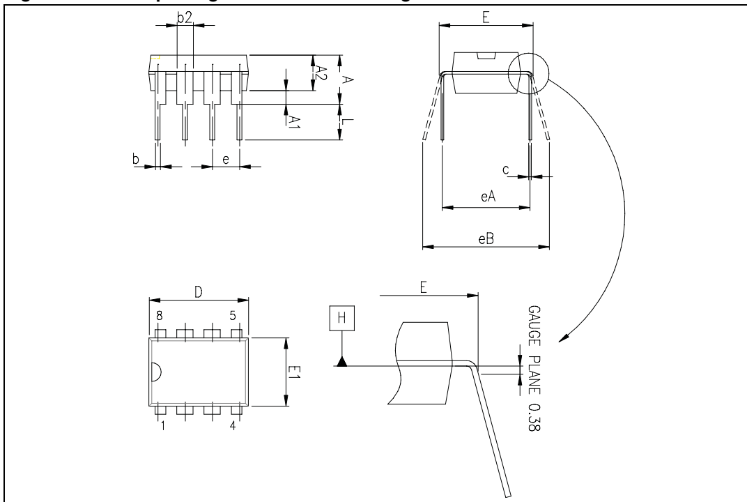
Figure 2. DIP8 package mechanical drawing
