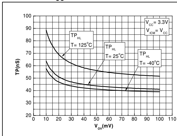
Figure 19. Propagation delay vs. overdrive V_{CC} = 3.3\text{ V}
