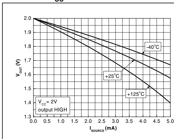
Figure 5. Output voltage vs. source current V_{CC} = 2V
