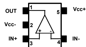
Pin connections (top view)
