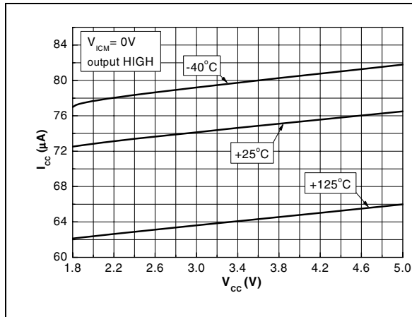
Figure 1. Current consumption vs. power supply voltage
