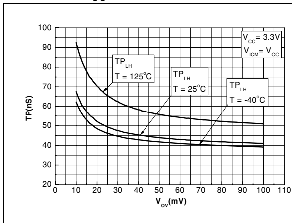
Figure 21. Propagation delay vs. overdrive V_{CC} = 3.3\text{ V}
