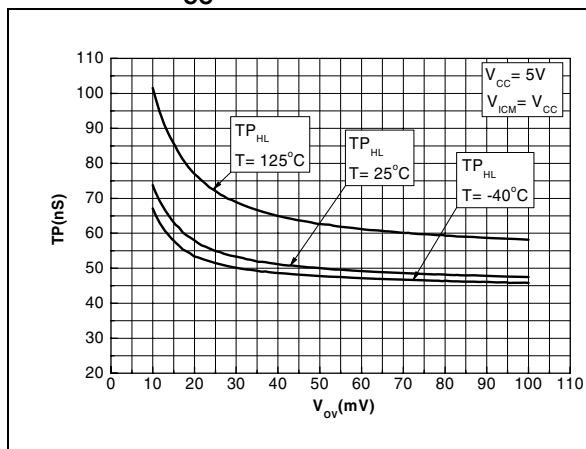
Figure 23. Propagation delay vs. overdrive V_{CC} = 5\text{ V}
