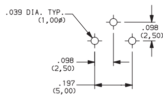
PC MOUNTING
