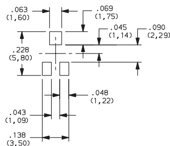
PC MOUNTING
