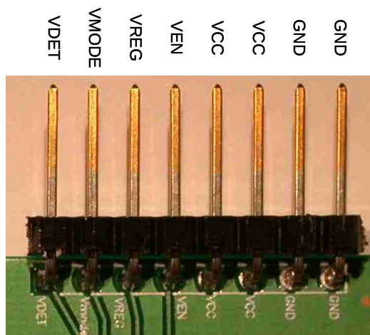
Single Row 8-position 0.1" Header Pins
