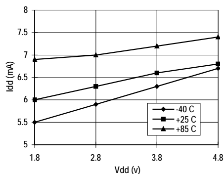
Idd vs. Vdd vs. Temperature
