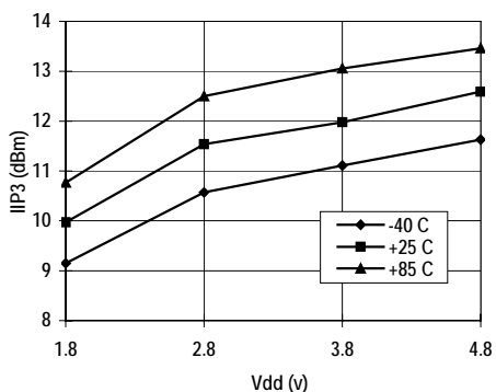
Input IP3 vs. Vdd vs. Temperature
