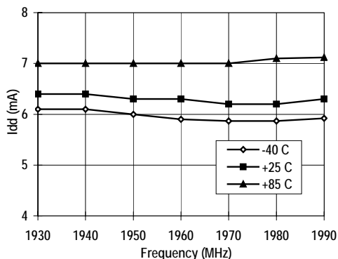
Idd vs. Temperature vs. Frequency
