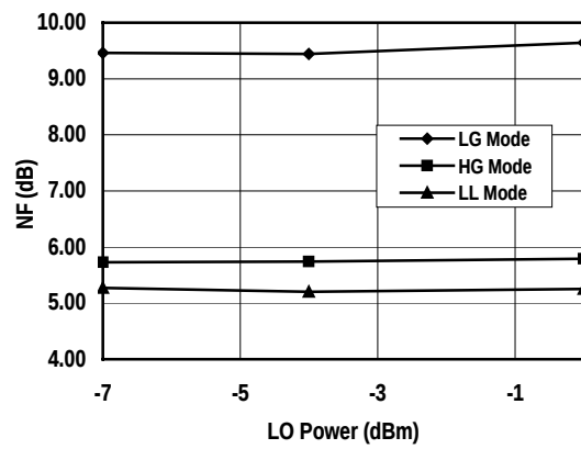
Noise Figure vs. LO Power
