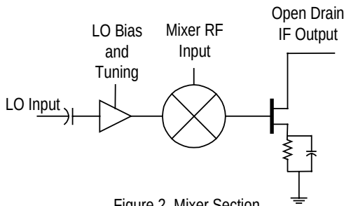
Figure 2, Mixer Section
