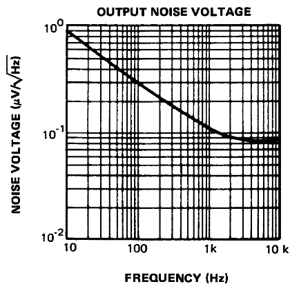
Figure 1 : Output Noise Voltage
