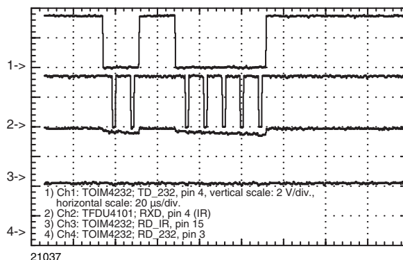
Figure 14. Echo-Suppression
