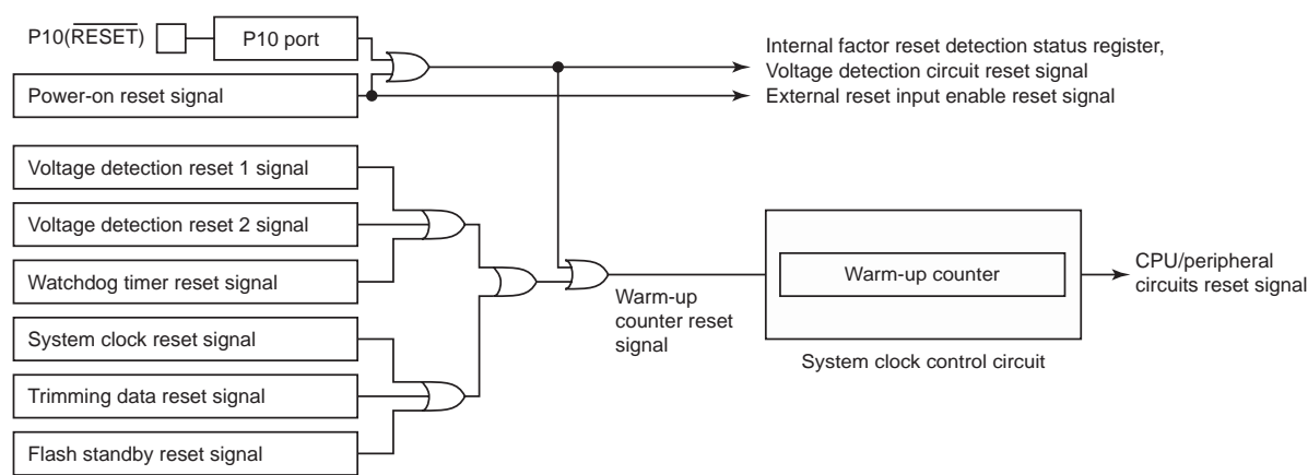
Figure 2-14 Reset Control Circuit
