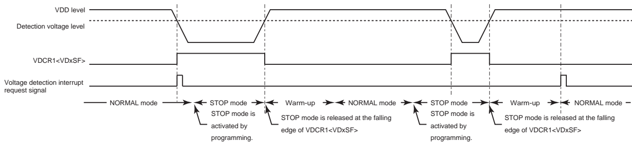
Figure 7-4 STOP Mode Release by VDCR1<VDxSF>
