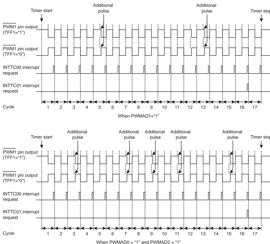
Figure 14-13 Examples of Inserting Additional Pulses
