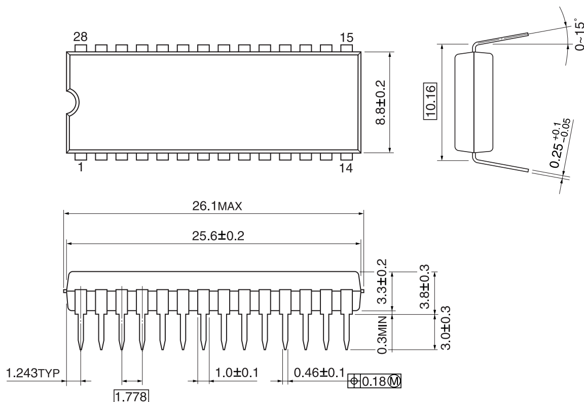
P-SDIP28-400-1.78
