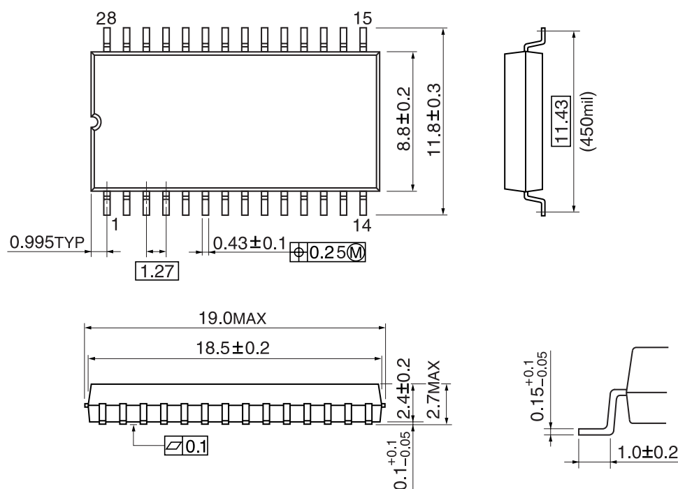
P-SOP28-450-1.27
