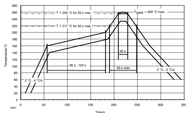
Figure 2. Solder Profile, RSS Recommendation
