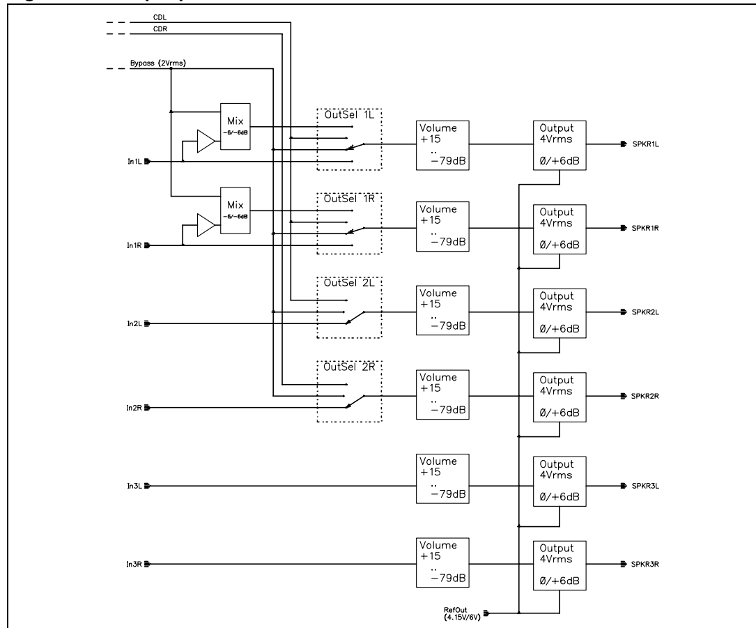
Figure 10. Output part.
