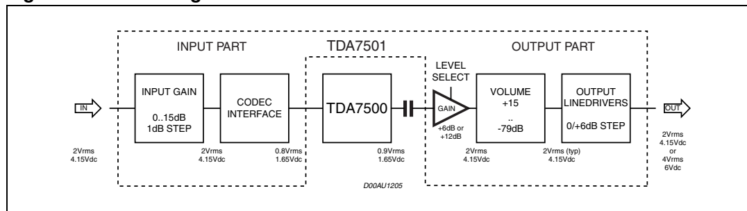
Figure 11. Level diagram.
