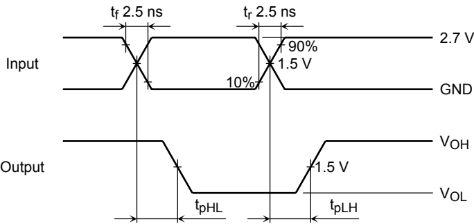
Figure 2 t_{pLH} , t_{pHL}
