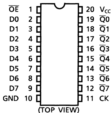
TC74HC564A
