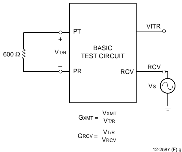
Figure 8. ac Gains
