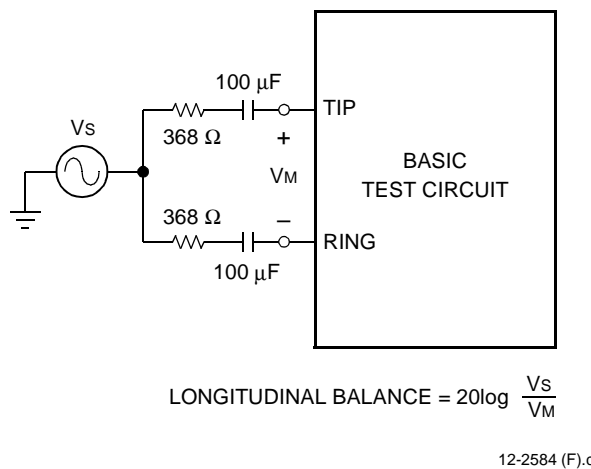
Figure 7. Longitudinal Balance
