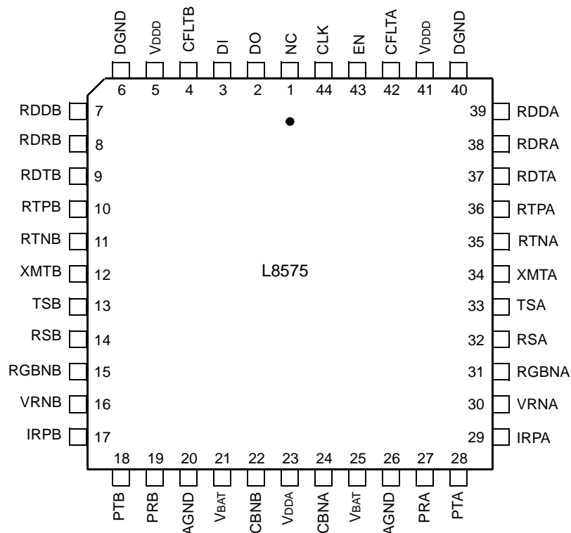
Figure 2. 44-Pin PLCC Pinout
