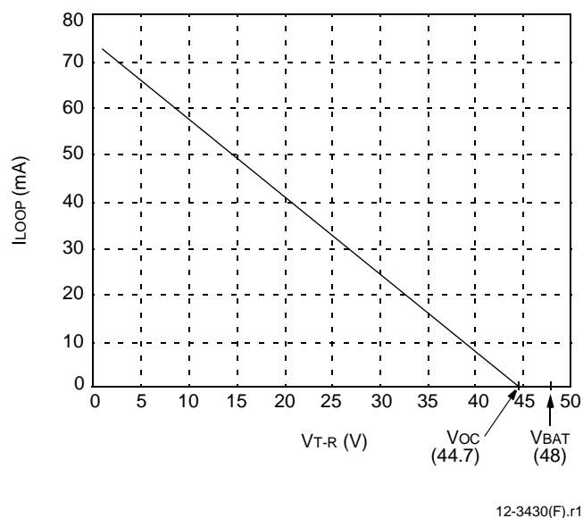
Figure 11. L8575 SLIC I/V Template
