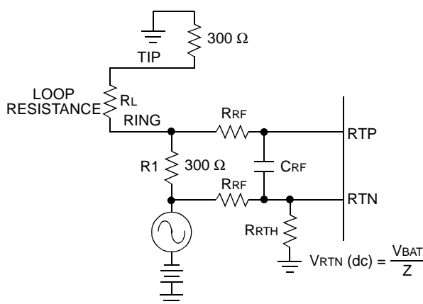
Figure 9. Ring-Trip Threshold
