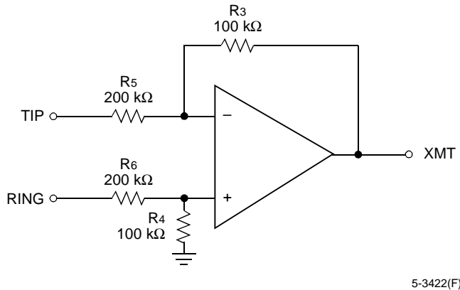
Figure 5. L8575 SLIC Dual-Resistive Matching Requirements
