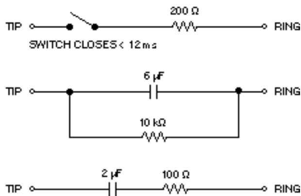
Figure 10. Ring-Trip Circuits
