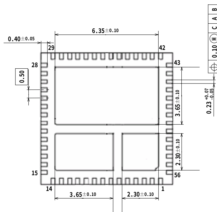
Bottom View
