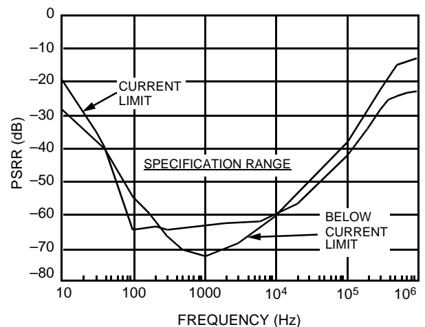
Figure 16. Typical V BAT Power Supply Rejection
