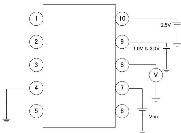
(3) Output dynamic range (Low side)(High side)
