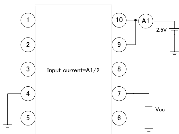
(2) OP-AMP1 Input current
