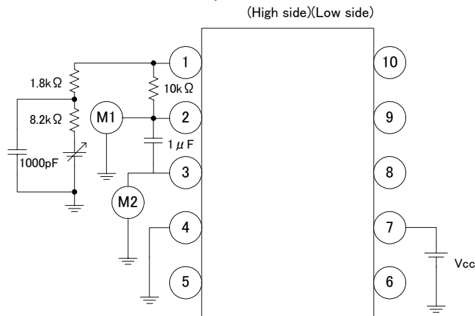
(16)Window-Comparator Detection voltage level (High side)(Low side)
