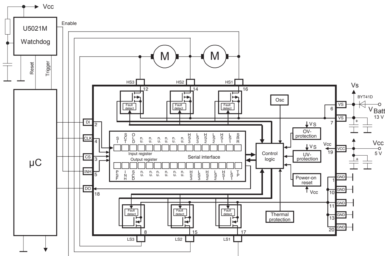
Figure 10-1. Application Circuit
