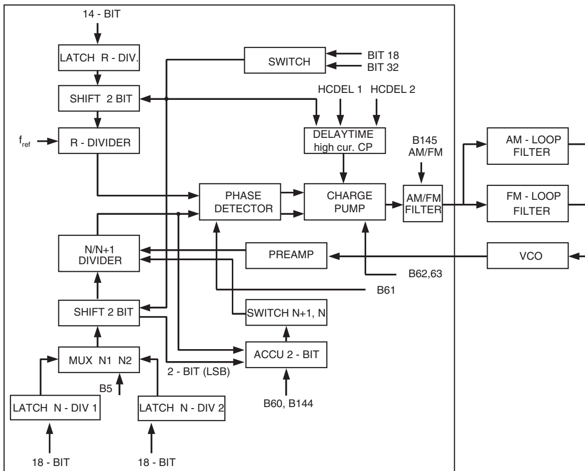
Figure 11-3. Block Diagram of the PLL Core
