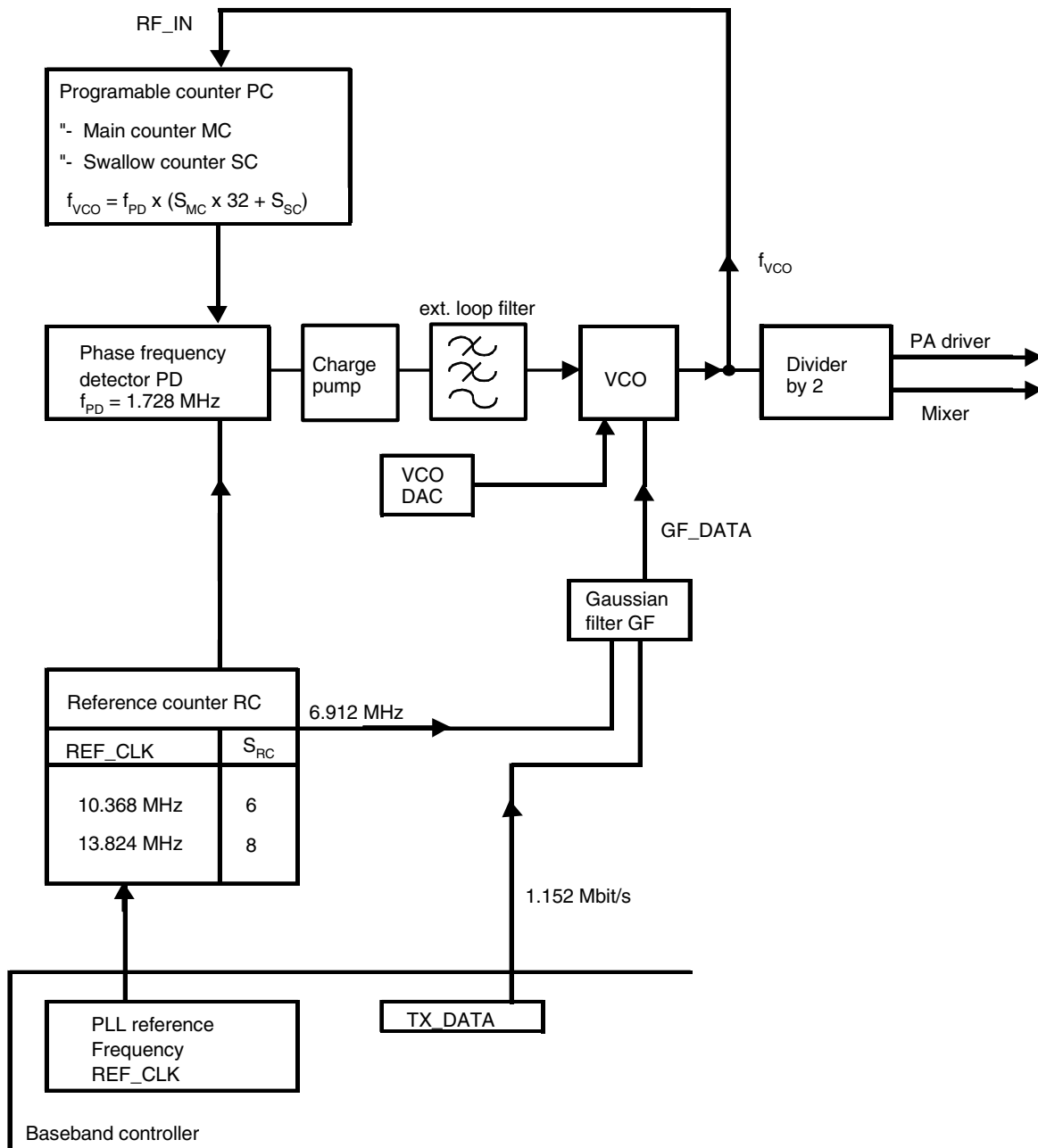
Figure 3-1. PLL Principle
