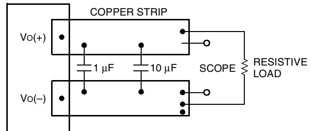
Figure 15. Input Reflected-Ripple Test Setup
