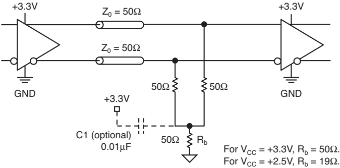
Figure 4b. Parallel Termination (3-Resistors)
