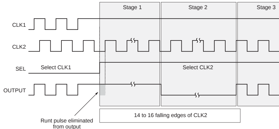
Figure 3. Timing Diagram 2 (1)
