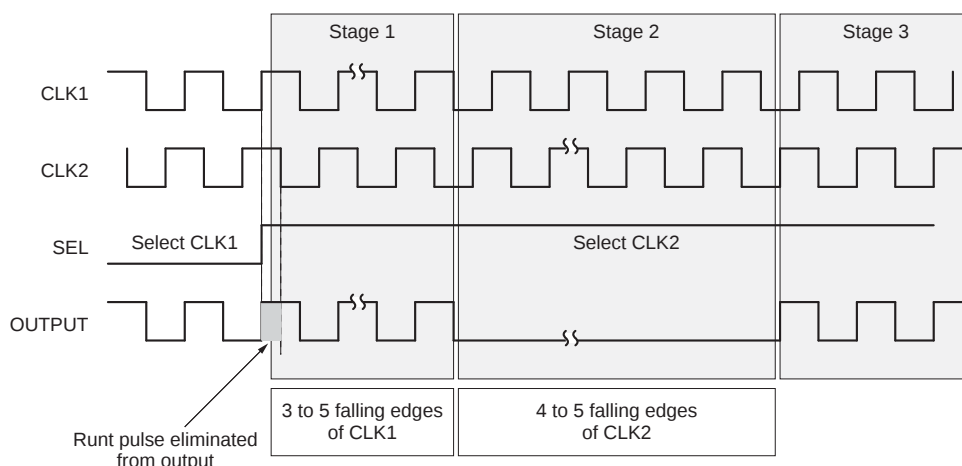
Figure 2. Timing Diagram 1
