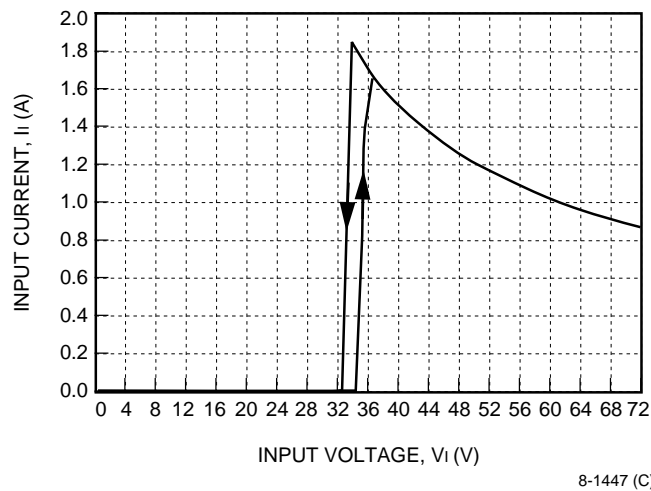
Figure 2. Typical JW075F Input Characteristics at Room Temperature
