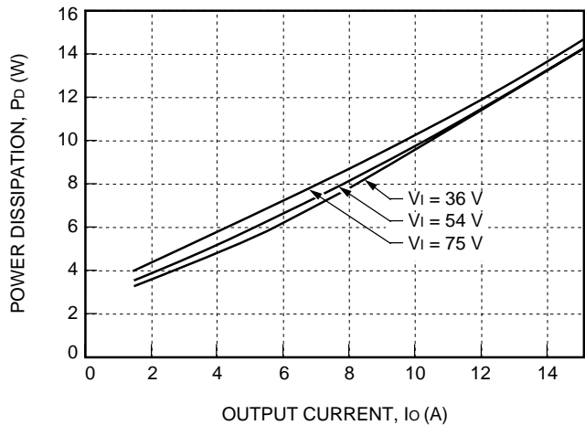
Figure 28. JW075F Power Dissipation vs. Output Current
