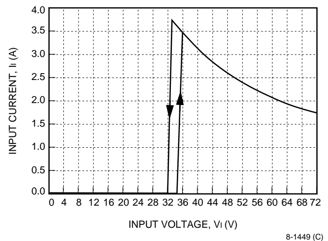
Figure 4. Typical JW150F Input Characteristics at Room Temperature
