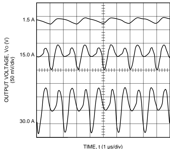
Figure 13. Typical JW150F Output Ripple Voltage at Room Temperature, I_o = Full Load
