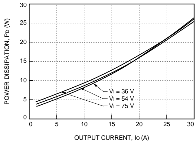
Figure 30. JW150F Power Dissipation vs. Output Current
