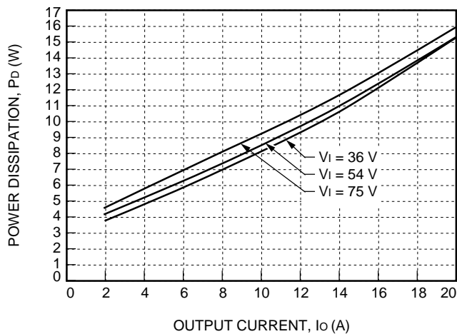
Figure 29. JW100F Power Dissipation vs. Output Current
