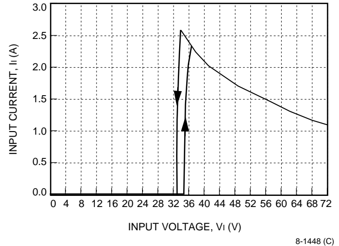
Figure 3. Typical JW100F Input Characteristics at Room Temperature
