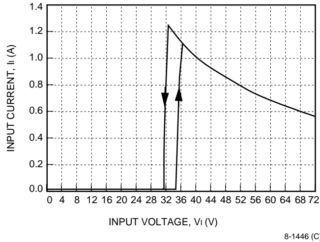
Figure 1. Typical JW050F Input Characteristics at Room Temperature
