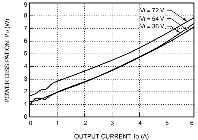
Figure 31. JW030A-M Power Dissipation vs. Output Current
