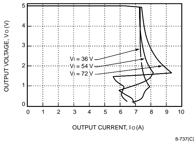
Figure 6. JW030A-M Typical Output Characteristics
