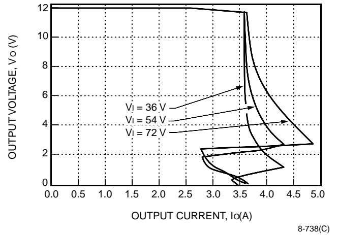
Figure 7. JW030B-M Typical Output Characteristics
