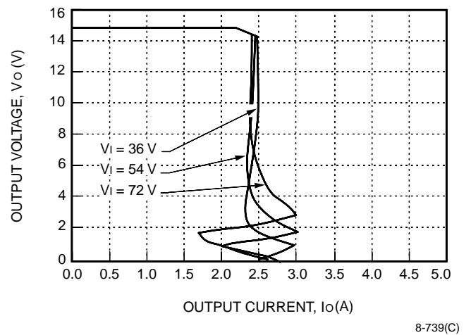
Figure 8. JW030C-M Typical Output Characteristics
