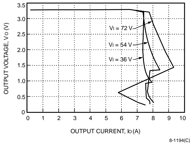
Figure 5. JW030F-M Typical Output Characteristics
