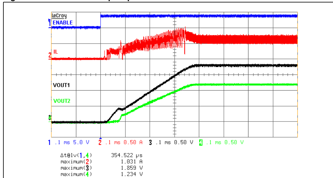
Figure 2. Smooth start-up sequence
