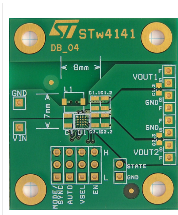
Figure 16. Demoboard top layer
