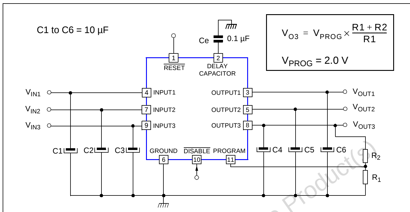
Figure 4: STV8164 Typical Application
