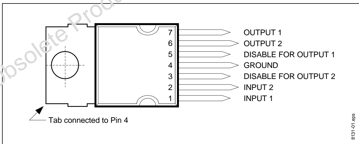
Figure 1. Pin Connections
