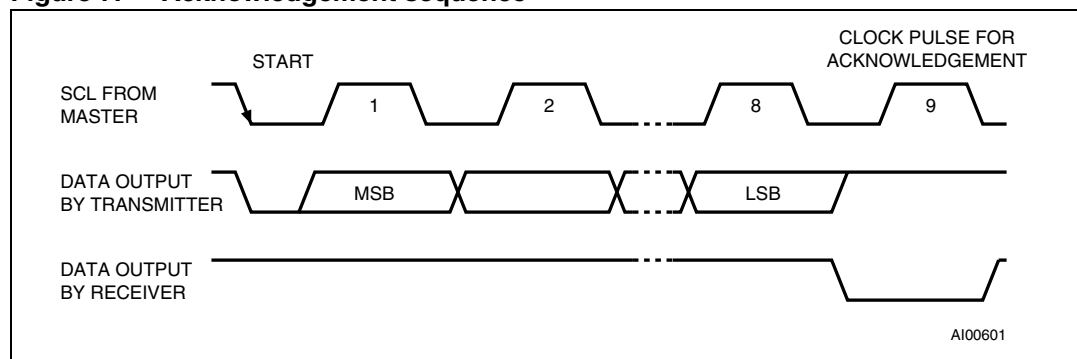
Figure 7. Acknowledgement sequence
