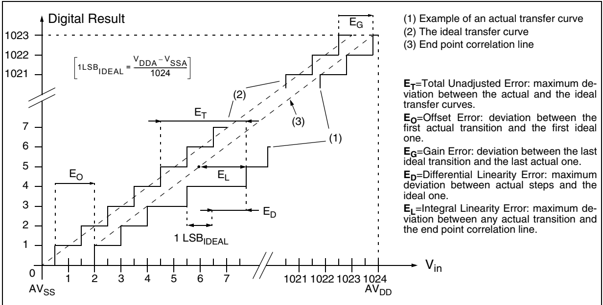
Figure 33. ADC conversion characteristics
