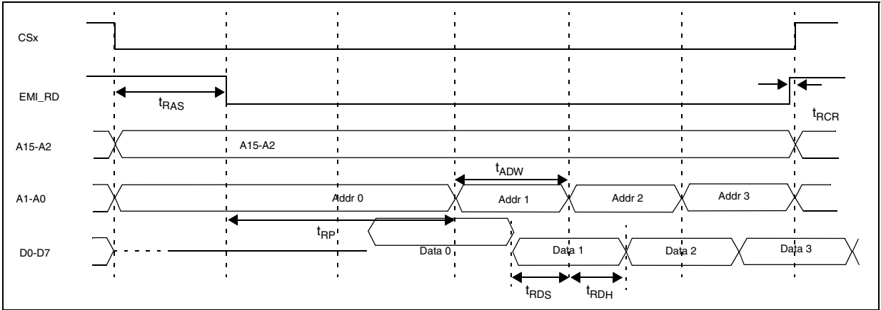
Figure 22. Page mode read diagram
