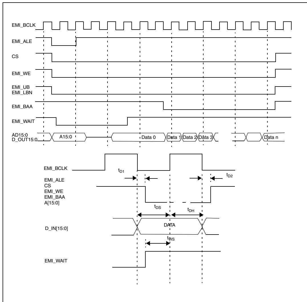
Figure 23. Sync burst write diagram
