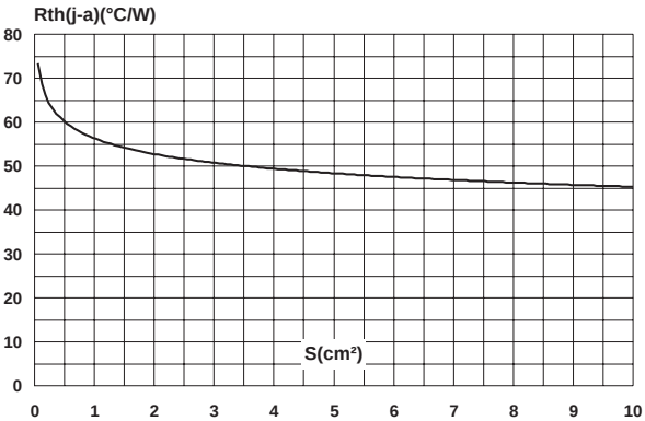
Fig. 10: Thermal resistance junction to ambient versus copper surface under each lead (epoxy printed board FR4, Cu = 35 \mu\text{m} ).
