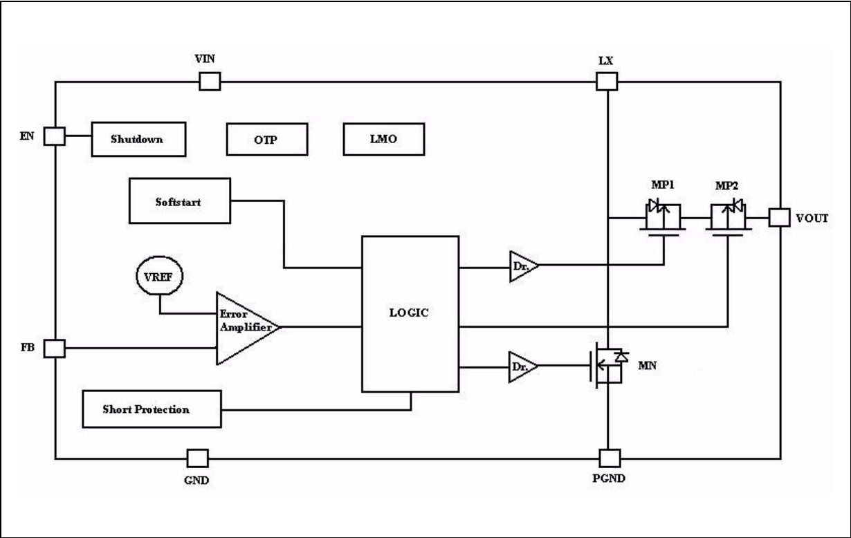
Figure 1. Internal block diagram
