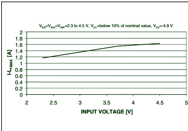
Figure 9. Step-up inductor peak current vs input voltage
