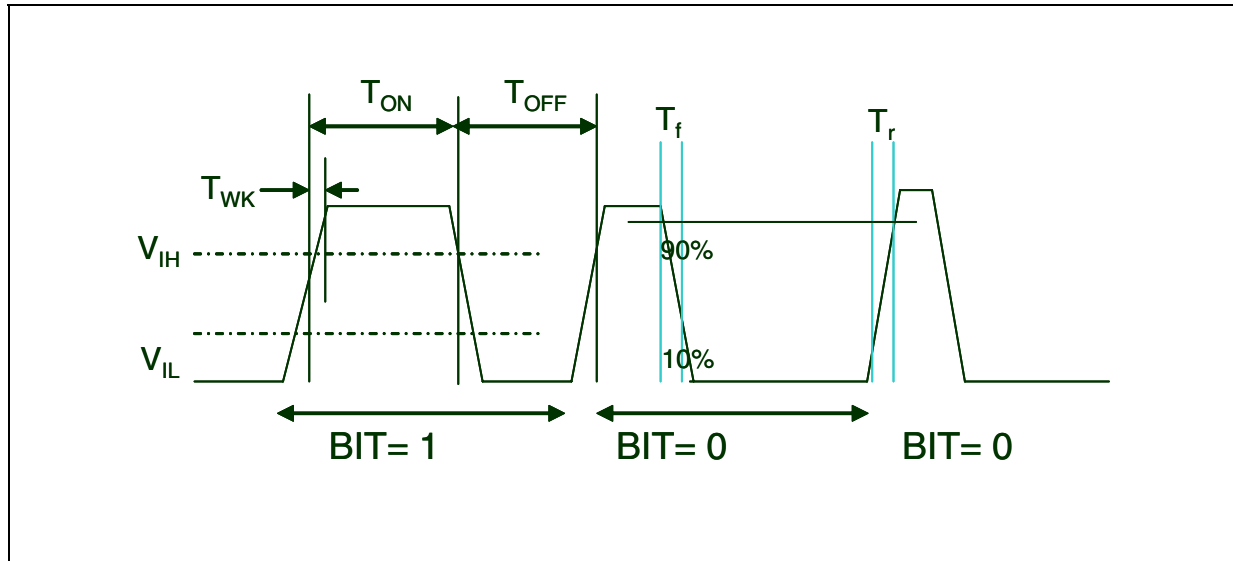
Figure 5. Waveform
