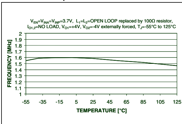
Figure 11. PWM step-up frequency vs temperature
