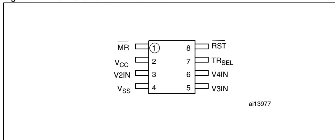
Figure 2. MSOP/TSSOP-8 connections
