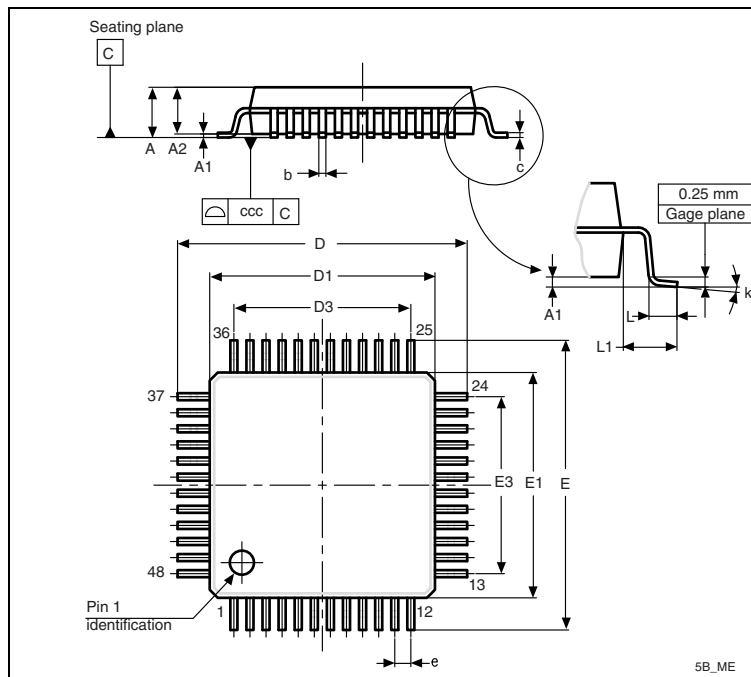
Figure 31. LQFP48 – 48-pin low-profile quad flat package outline (1)
