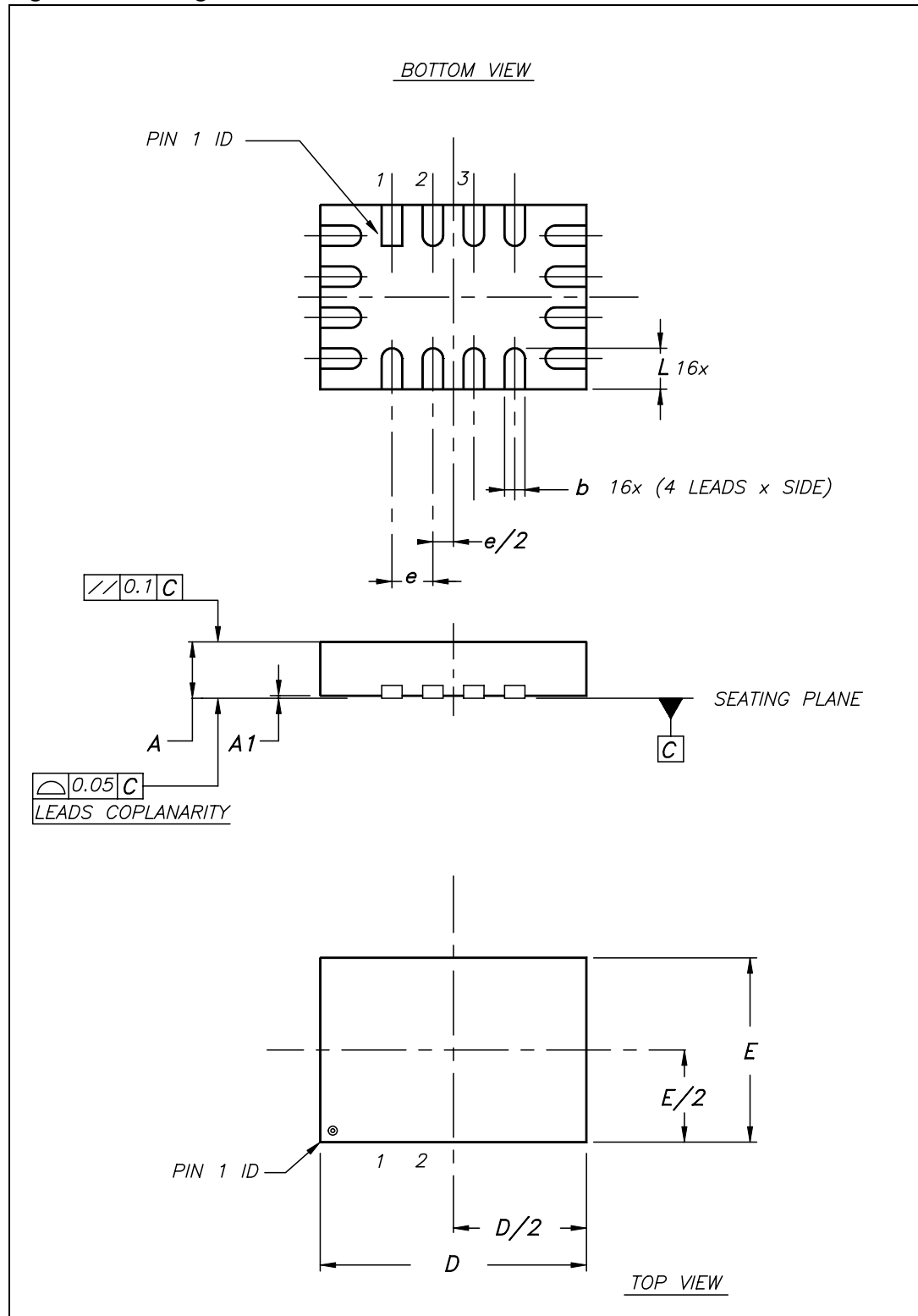
Figure 5. Package information
