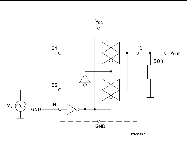
Figure 6. Channel-to-channel crosstalk
