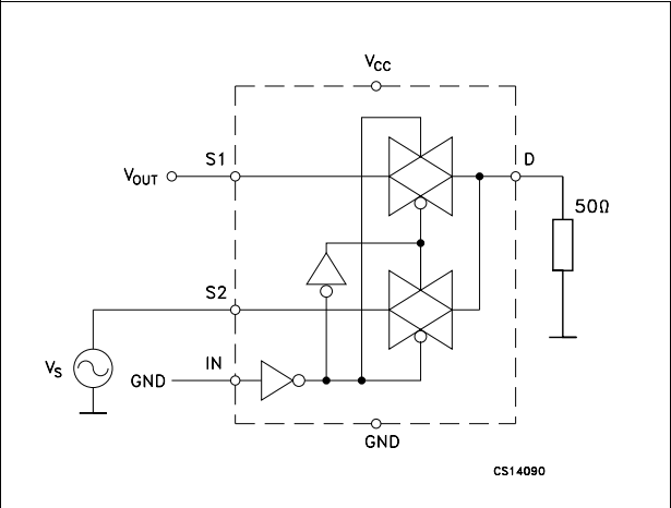
Figure 6. Channel-to-channel crosstalk
