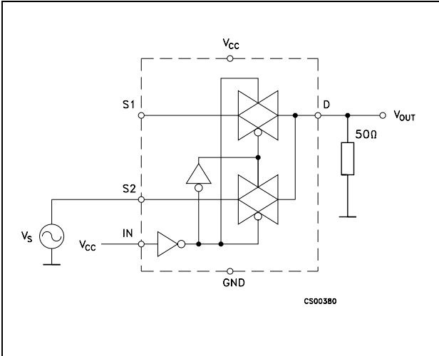
Figure 7. OFF Isolation
