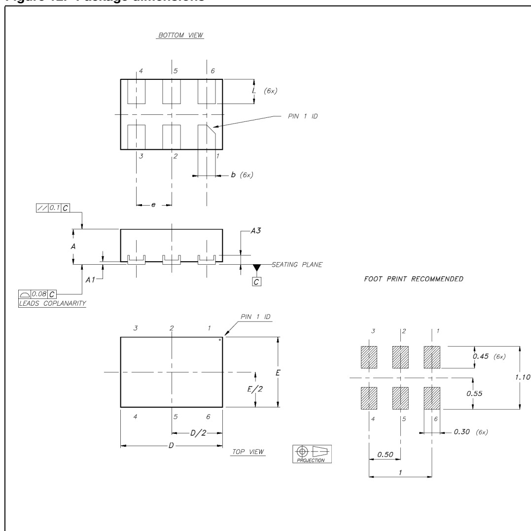
Figure 12. Package dimensions
