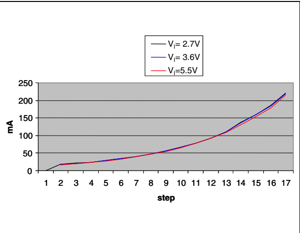
Figure 18. I_{OAUX} vs AUX1
