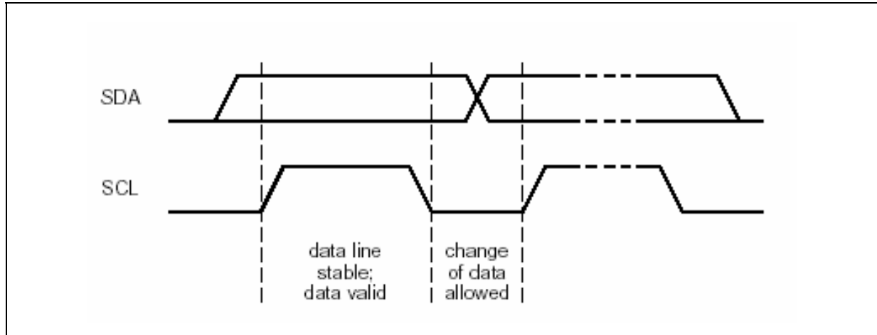
Figure 7. Bit transfer
