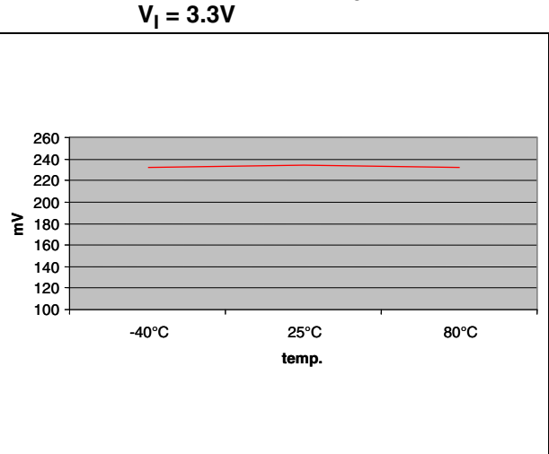
Figure 20. V_{FB2} vs Temp. at I_O = 800\text{mA} , V_1 = 3.3\text{V}
