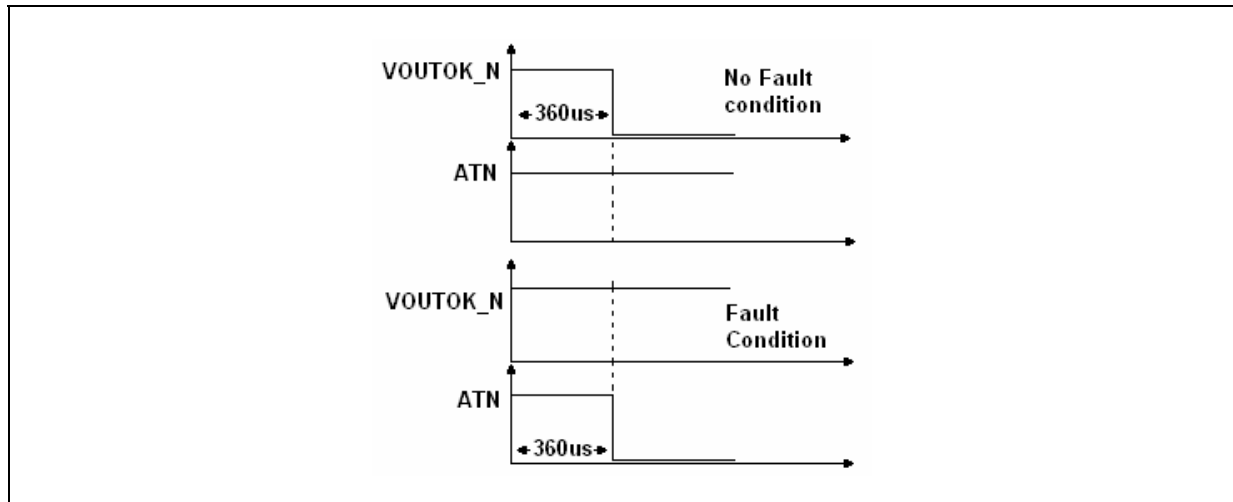
Figure 14. VOUTOK_N behavior
