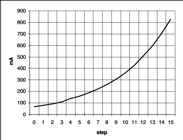
Figure 17. Aux current vs AUXI
