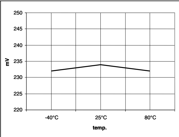
Figure 19. VFB2 flash vs temp
