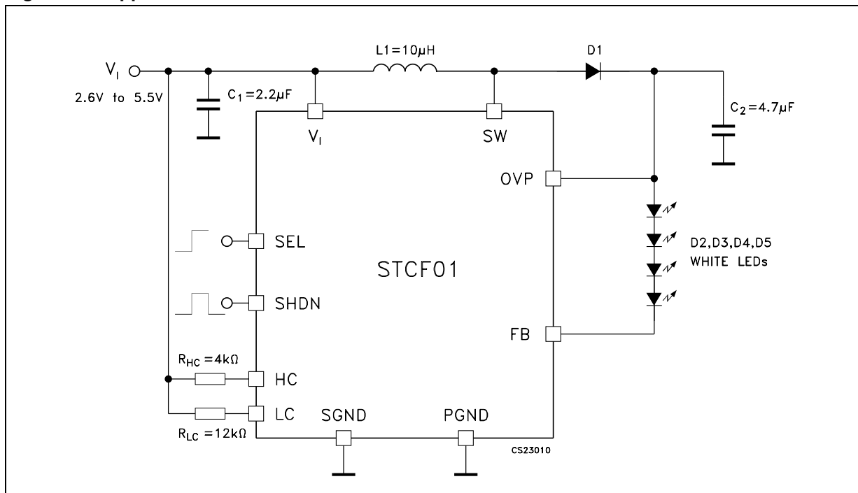
Figure 3. Application circuit
